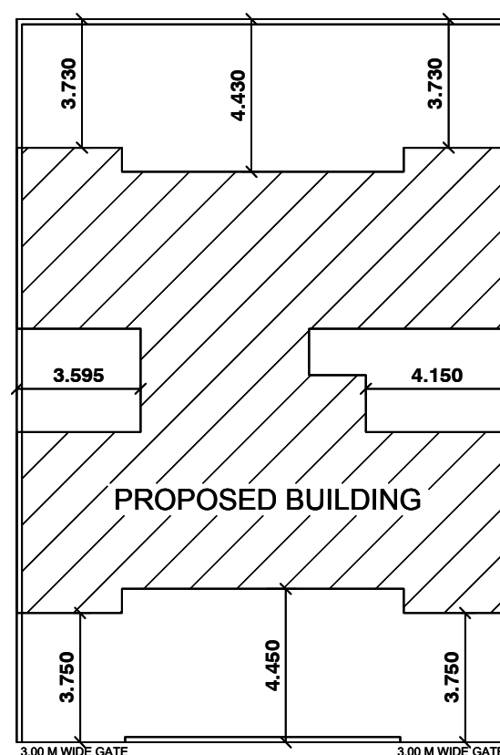
BLOCK PLAN
