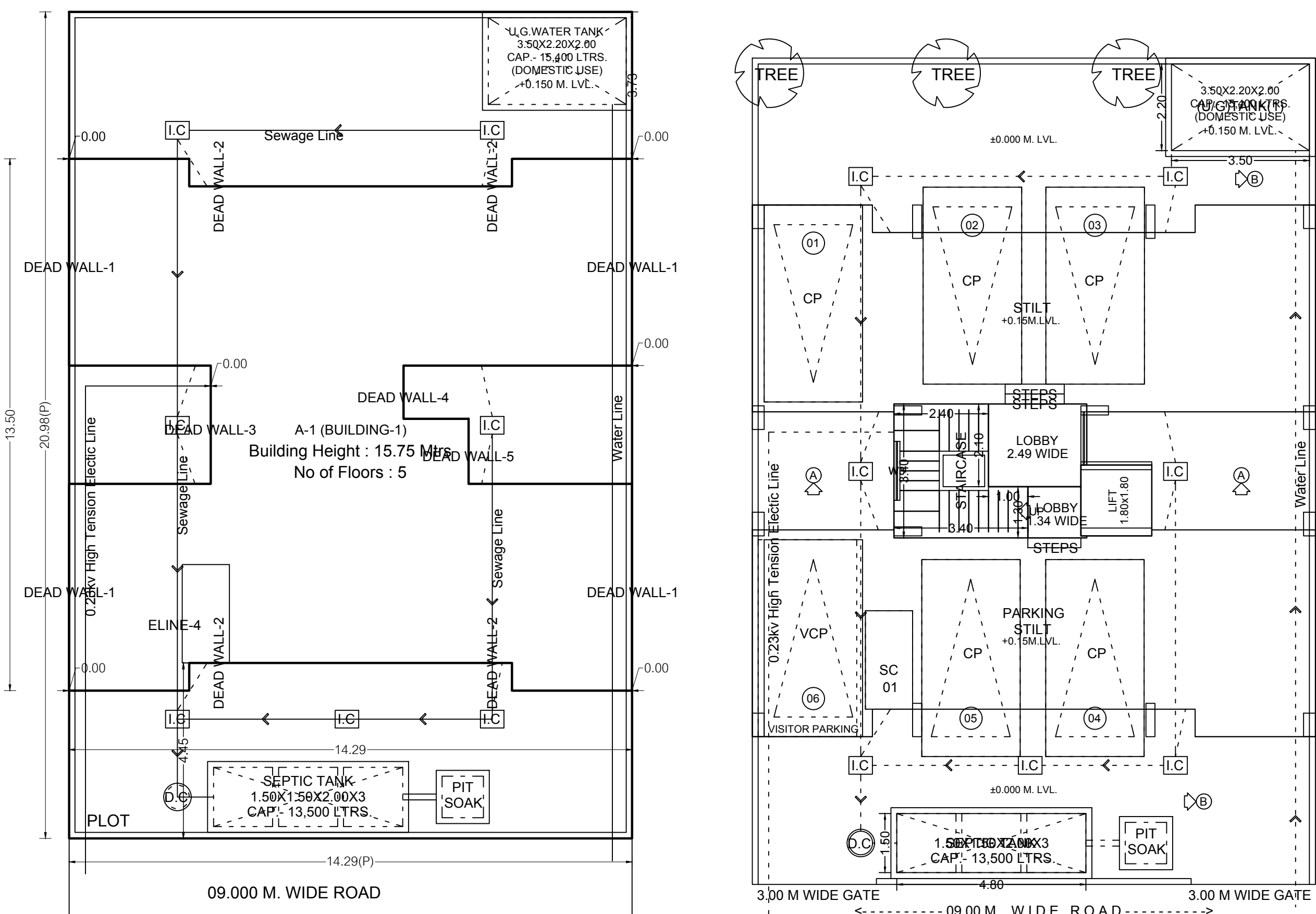
LAYOUT PLAN
