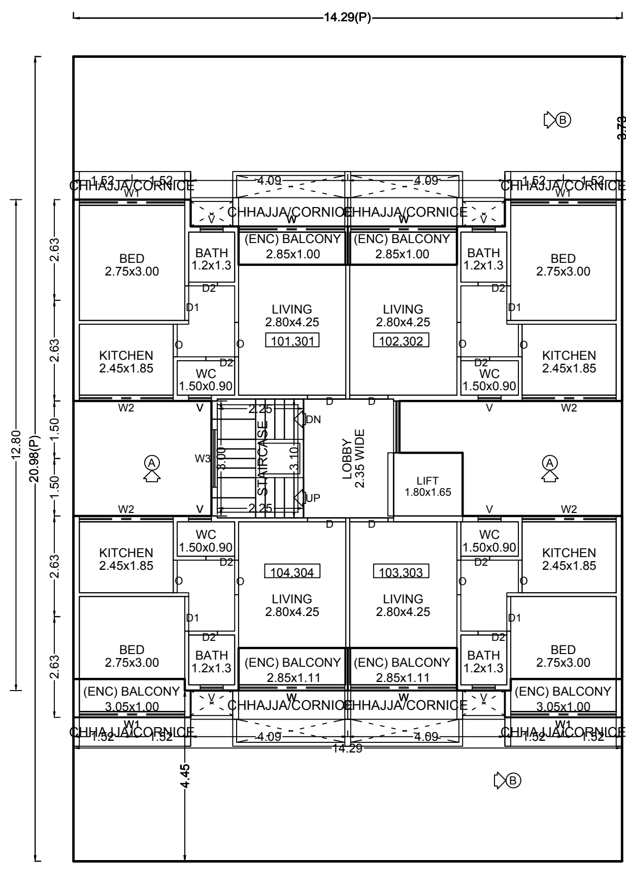
TYPICAL - 1 & 3 FLOOR PLAN
